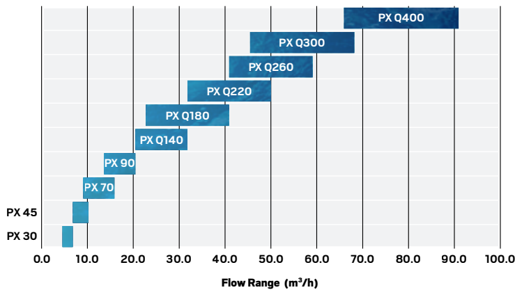
PX Q Series Flow Rates
